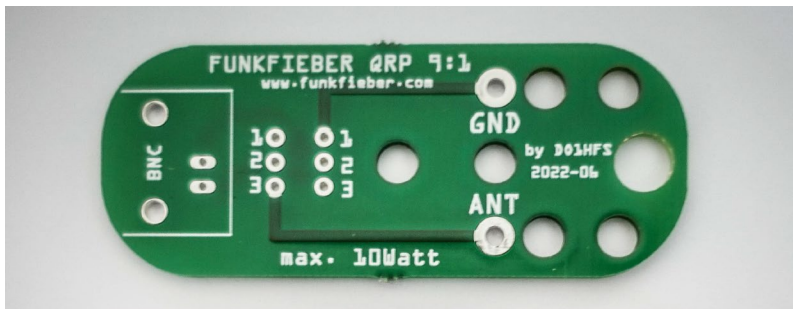
←V1.0 Platine
