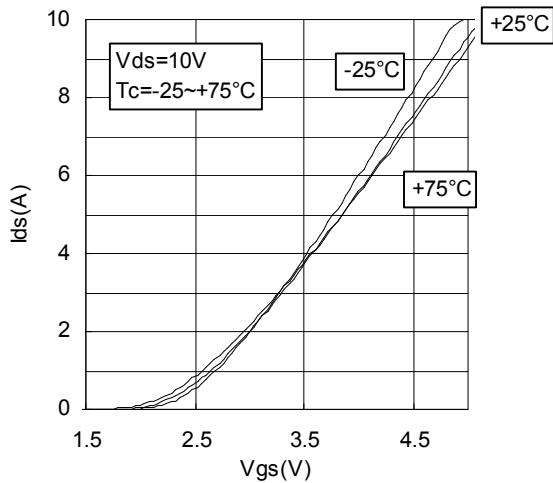
Vgs-Ids CHARACTERISTICS 2
