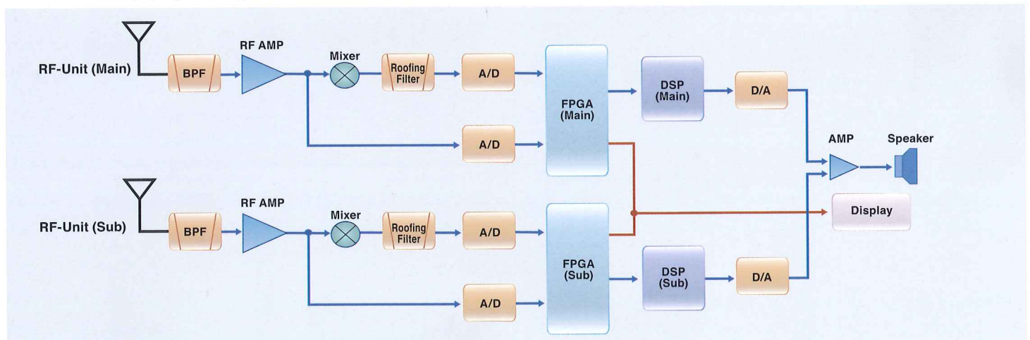
Completely Independent Dual Hybrid SDR System
