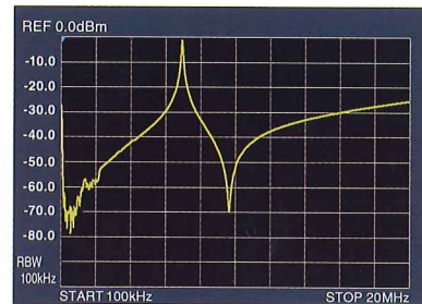
VC-TUNE characteristics
