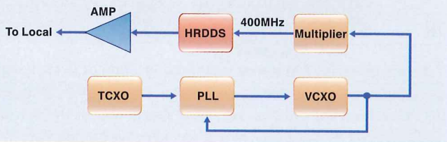
Local Oscillator block diagram
